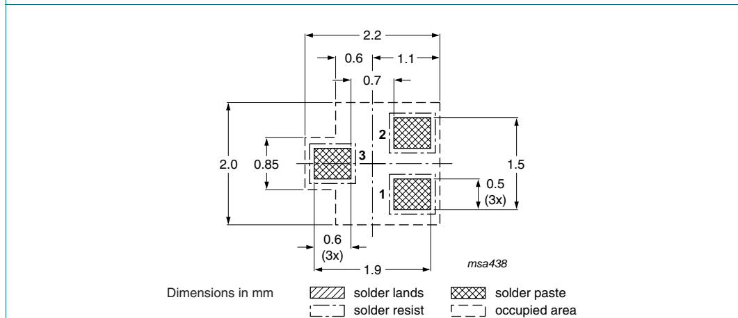
Fig 19. Reflow soldering footprint SOT416 (SC-75)
