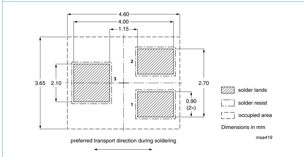
Fig 18. Wave soldering footprint SOT323 (SC-70)
