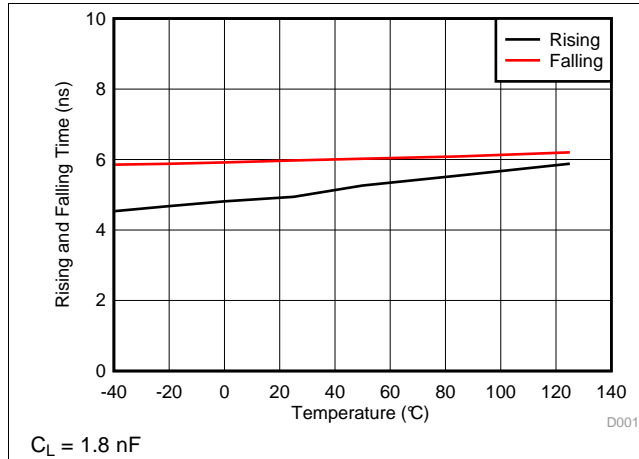
Figure 21. Rise Time and Fall Time
