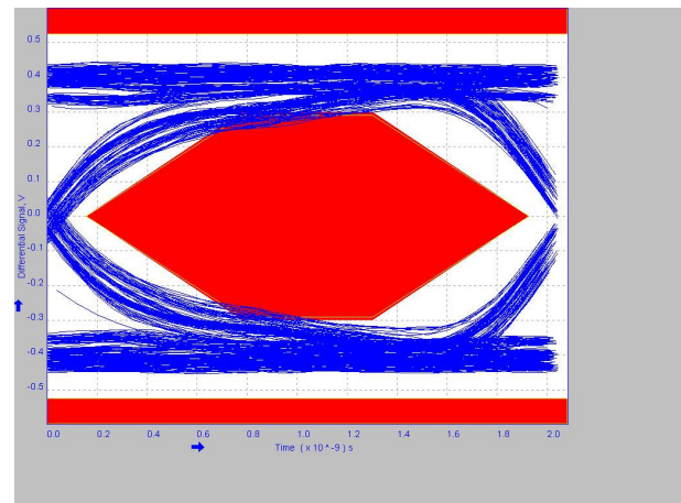
Figure 9-6. 3 Meter Pre-Channel Without TUSB217A
