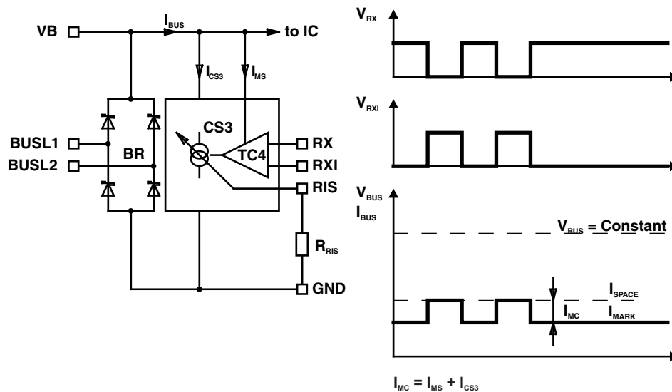
Figure 3. Data Transmission, Slave to Master
