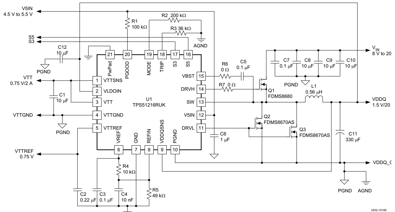
Figure 33. DDR3, 400-kHz Application Circuit, Tracking Discharge
