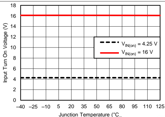
Figure 5. Input Turn-On Voltage vs. Junction Temperature
