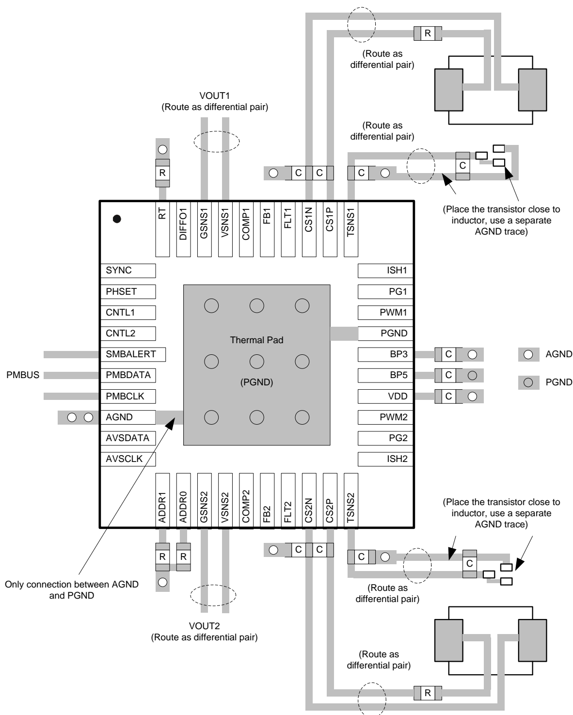
Figure 32. PCB Layout Recommendation
