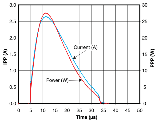
Figure 5. Pulse Waveform (8/20 \mu s Pulse)
