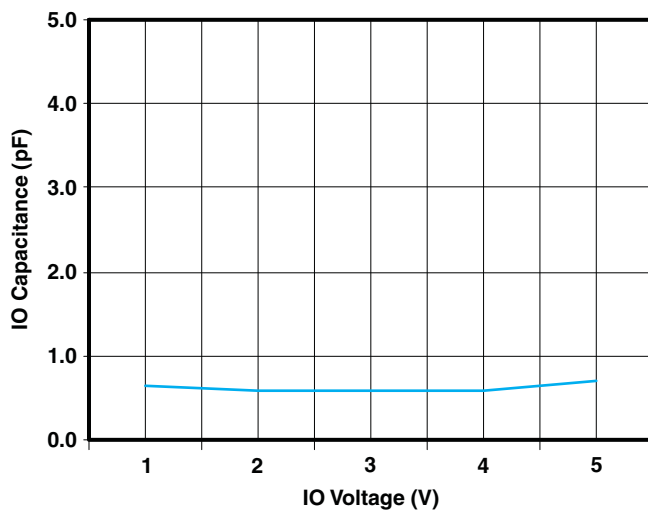
Figure 3. IO Capacitance vs Input Voltage ( V_{CC} = 5 V)
