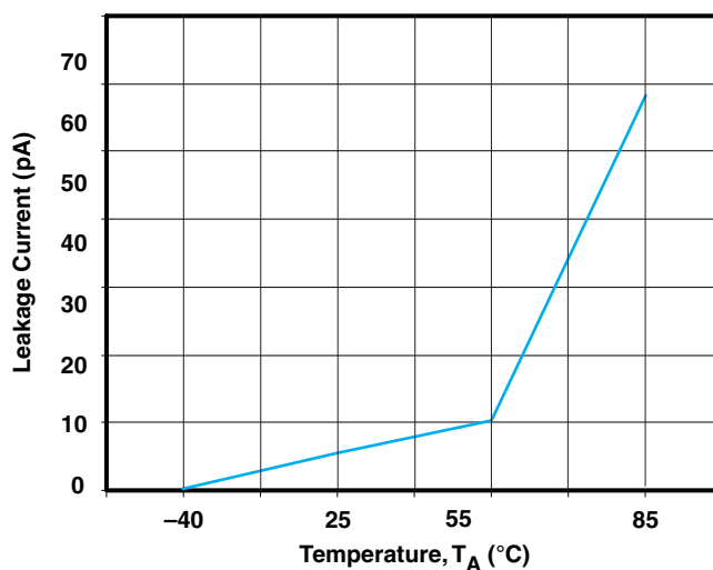
Figure 2. Leakage Current vs Temperature ( V_{I0} = 2.5 V)
