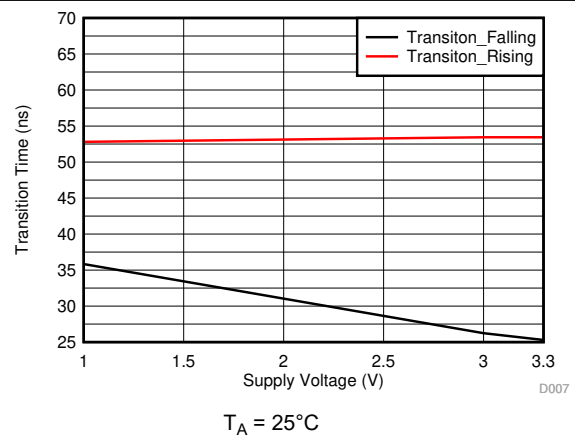
Figure 6-6. T_{\text{TRANSITION}} vs Supply Voltage
