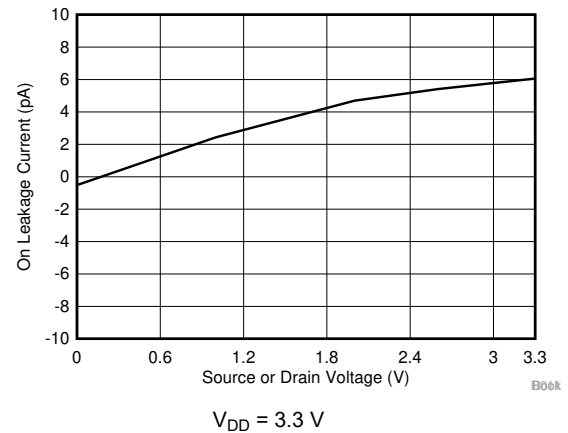
Figure 6-4. On-Leakage vs Source or Drain Voltage
