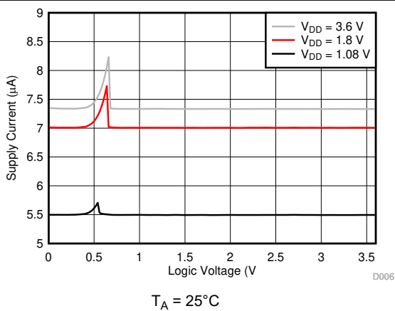
Figure 6-5. Supply Current vs Logic Voltage
