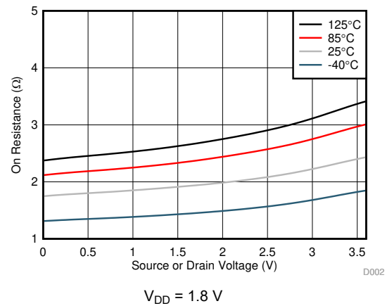
Figure 6-2. On-Resistance vs Temperature
