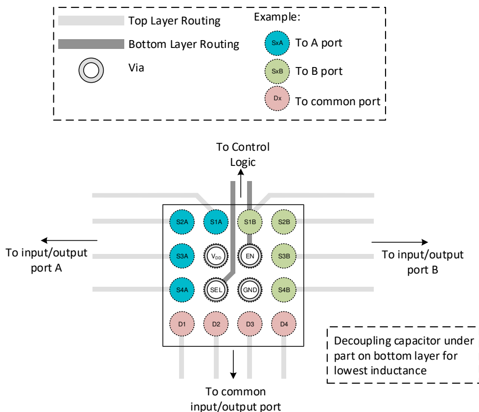
Figure 11-3. Example Layout
