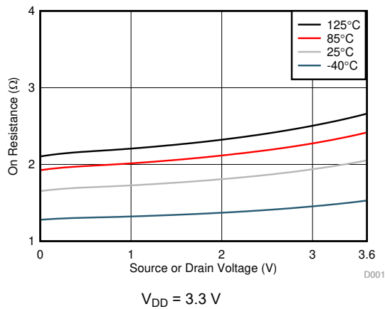
Figure 6-1. On-Resistance vs Temperature
