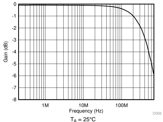
Figure 6. Frequency Response
