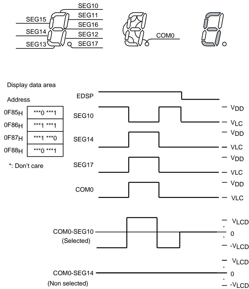
Figure 15-11 Static Drive
