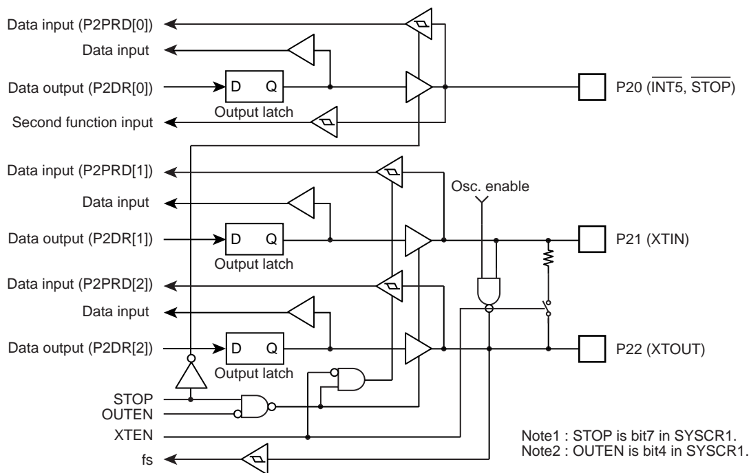
Figure 5-3 Port 2
