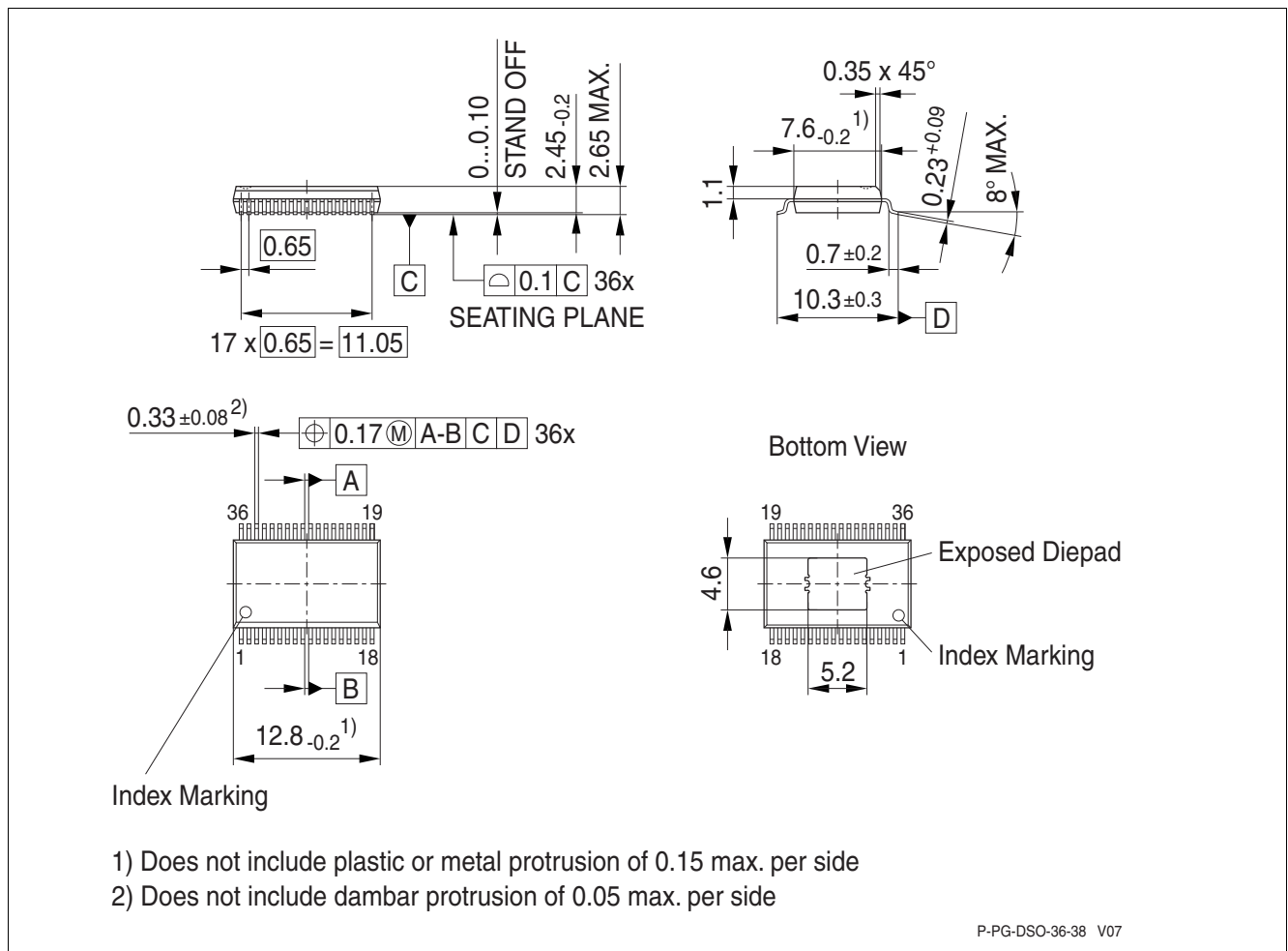
Figure 6 PG-DSO-36-38
