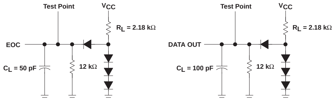
Figure 2. Load Circuits
