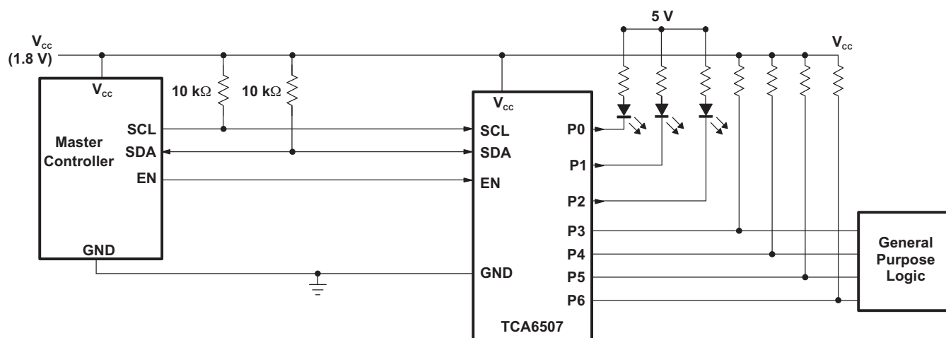
Figure 22. Typical Application
