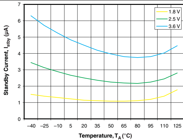
Figure 1. Standby Current vs Temperature [EN is Low (PWM Disabled), f SCL = 0]
