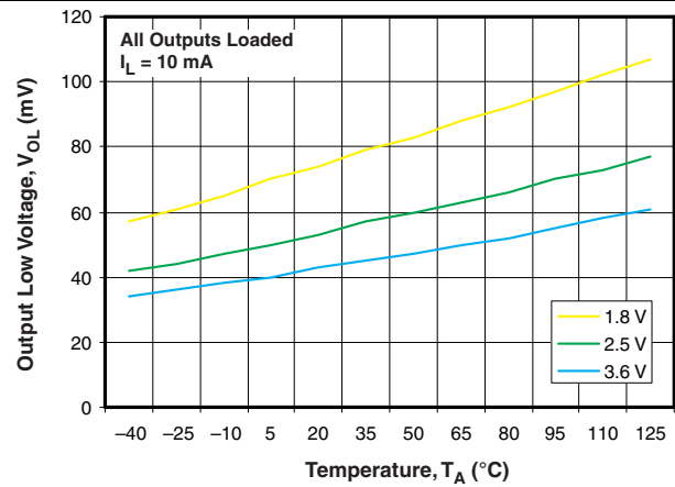
Figure 4. Port Output Low Voltage vs Temperature
