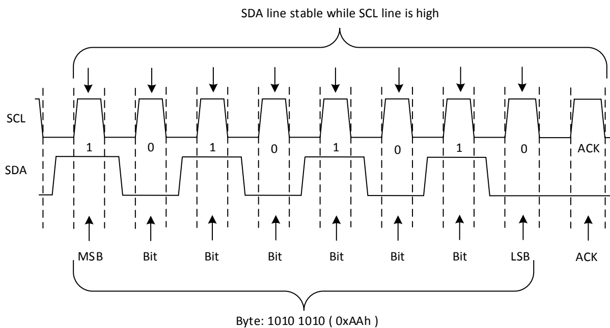
Figure 13. Bit Transfer
