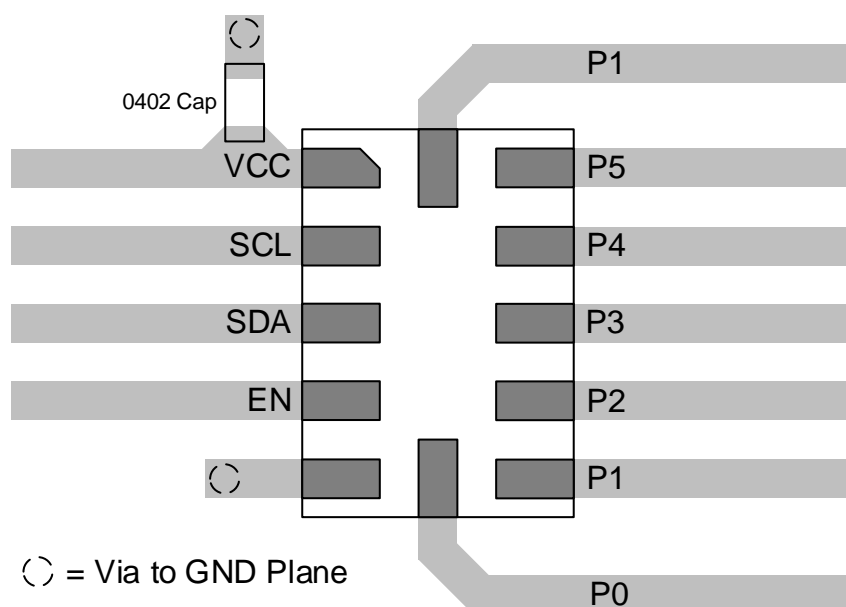
Figure 30. RUE Layout Recommendation
