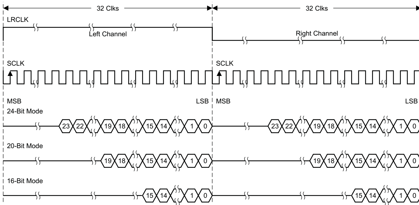
Figure 43. Right Justified 64\text{-}f_s Format
