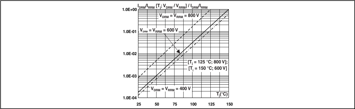
Figure 15. Relative variation of leakage current versus junction temperature for different values of blocking voltage
