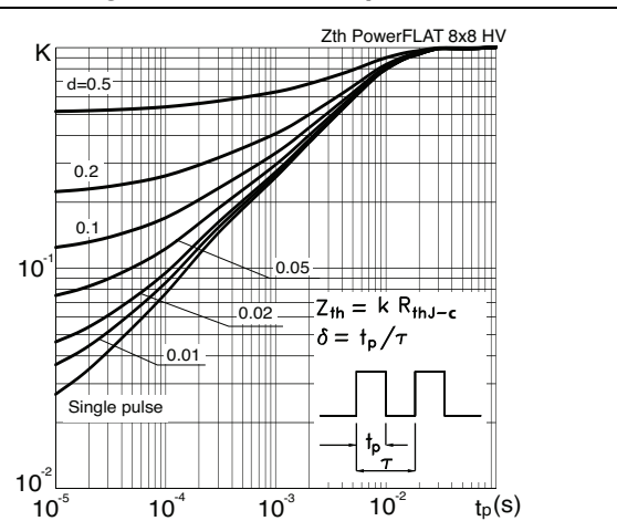
Figure 3. Thermal impedance
