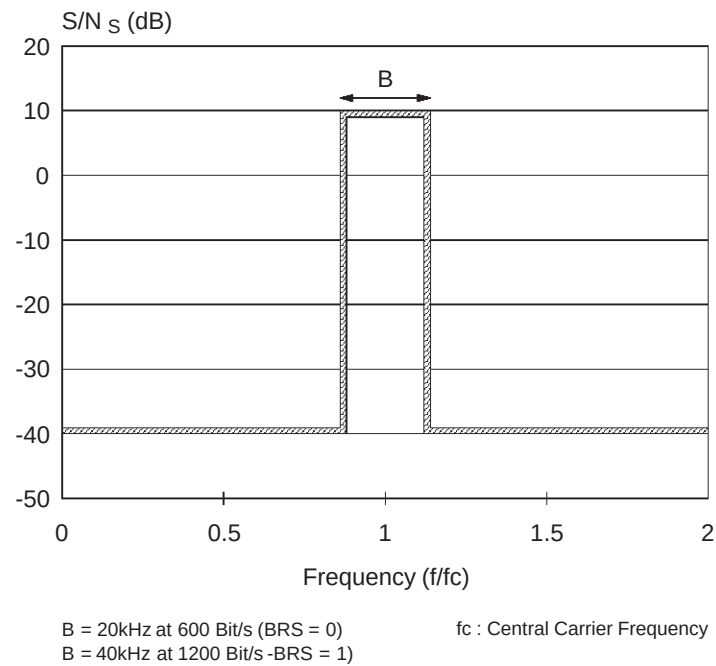
Figure 5 : S/N Mask for 80% AM Sine Noise
