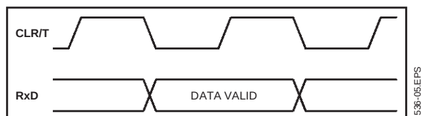
Figure 3 : Rx Data Output Timing
