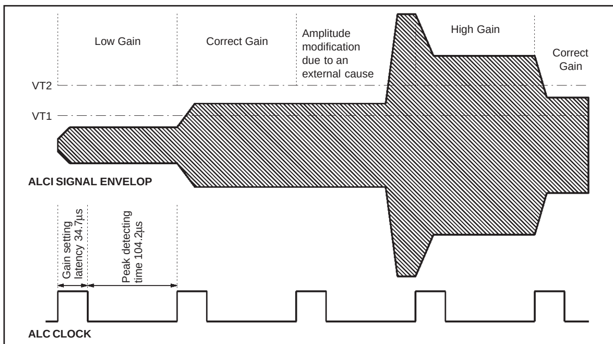
Figure 2 : Automatic Level Control Timing Chart
