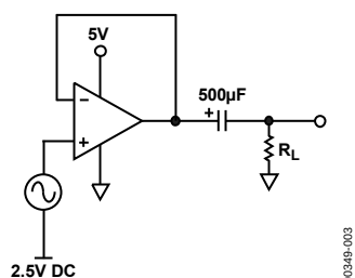
Figure 3. Test Circuit for Figure 4, Figure 5, and Figure 6
