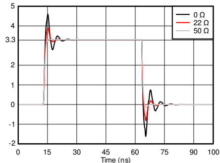
Figure 9-2. Application Timing Curve
