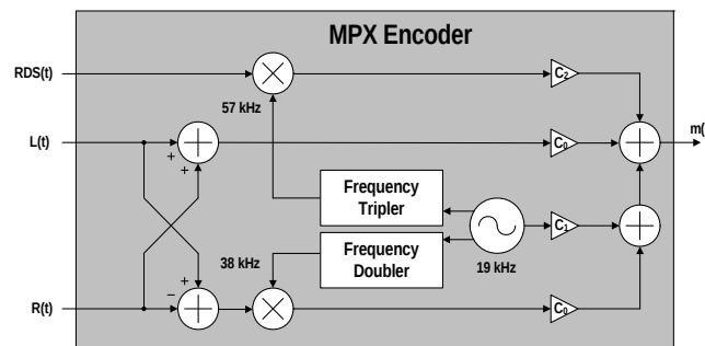
Figure 20. MPX Encoder
