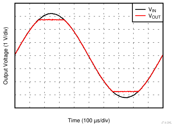
Figure 6-25. No Phase Reversal
