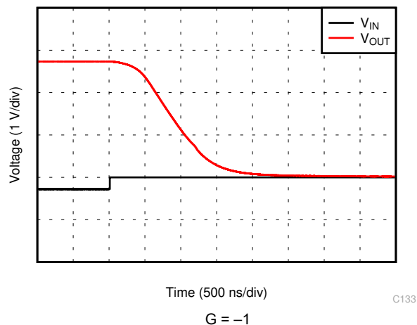
Figure 6-26. Overload Recovery
