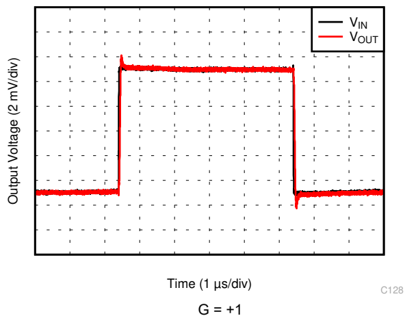
Figure 6-27. Small-Signal Step Response
