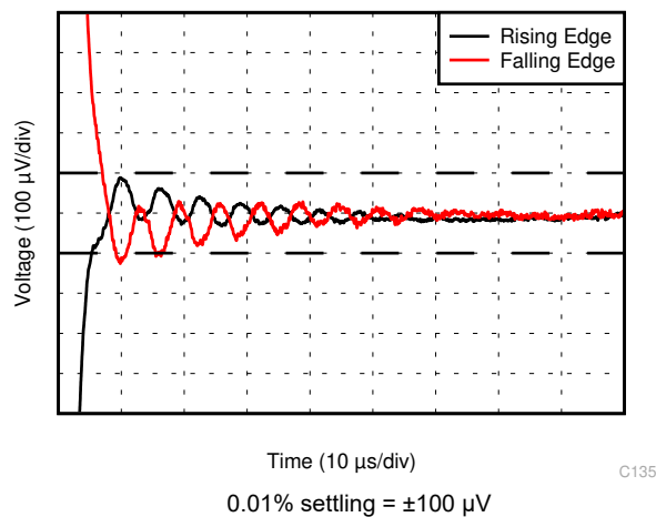
Figure 6-29. Settling Time
