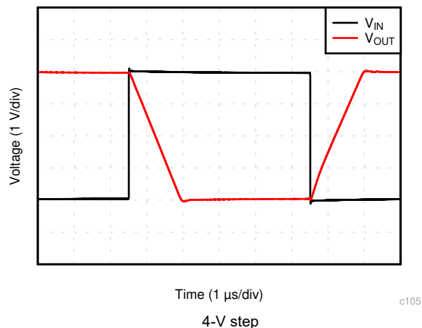
Figure 6-28. Large-Signal Step Response
