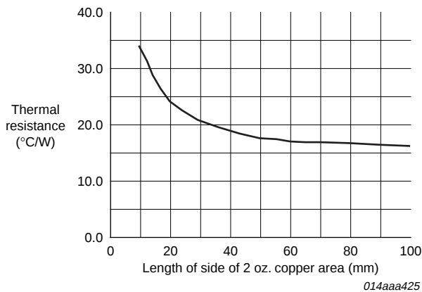
Fig 7. PCB heat sink area versus thermal resistance
