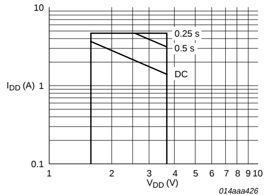
Fig 8. Safe operating area for the NE57810
