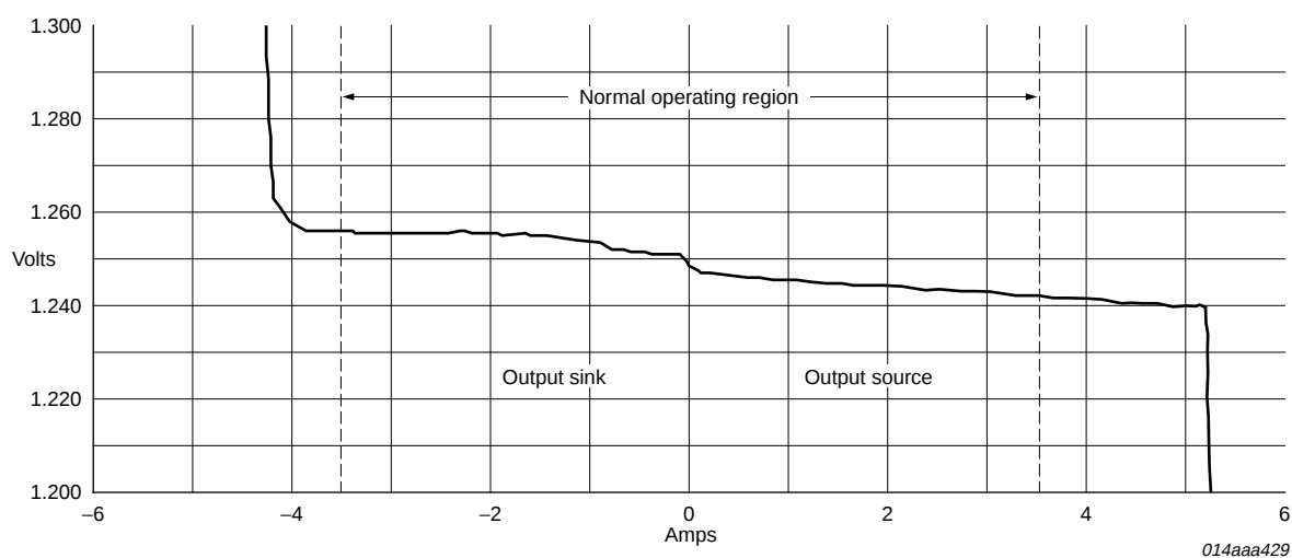
Fig 13. Typical V_{TT} versus output current ( V_{DD} = 2.5\text{ V} at 25\text{ °C} )
