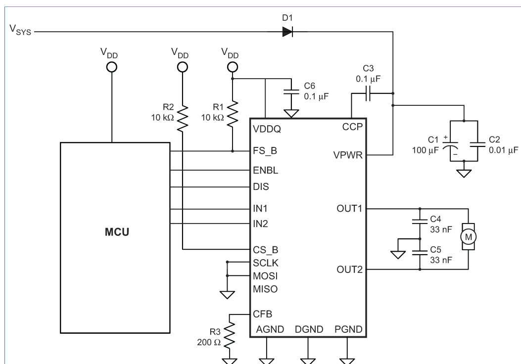
Figure 20. Simplified minimum application schematic (Reverse battery protection using a diode and operation without SPI)
