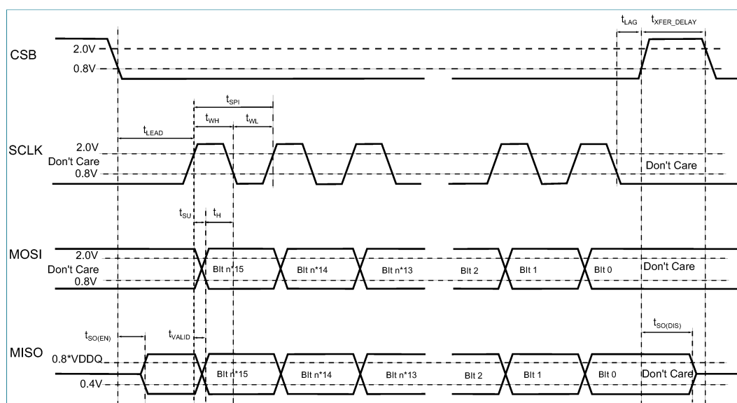
Figure 7. SPI dynamic diagram
