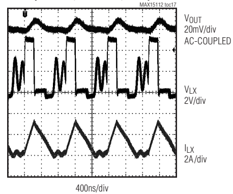
SWITCHING WAVEFORMS ( V_{IN} = 5V , I_{OUT} = 1A , SKIP)
