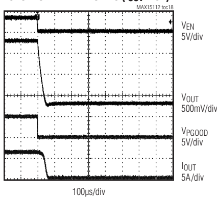
SHUTDOWN WAVEFORMS ( I_{OUT} = 6A )
