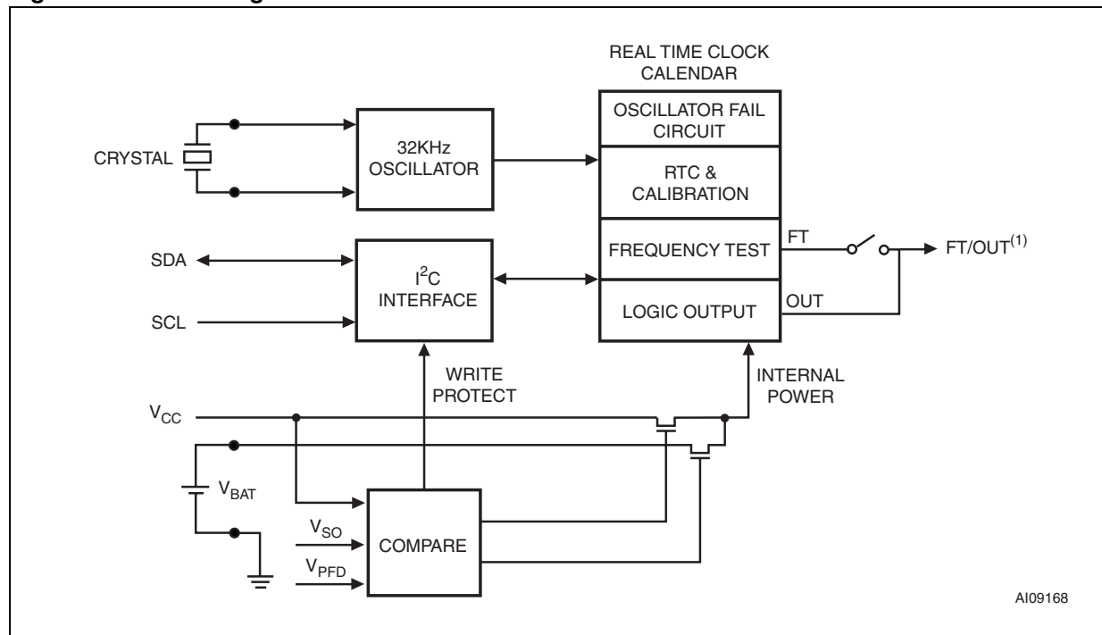
Figure 3. Block diagram
