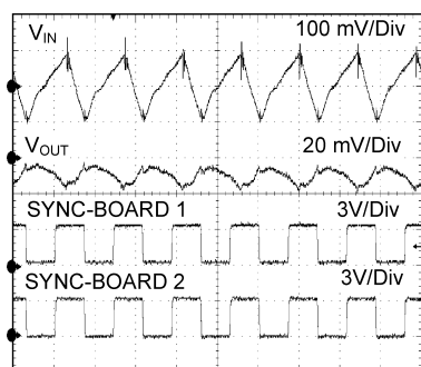
Figure 53. Output voltage ripple of two modules with synchronization clocks in phase
