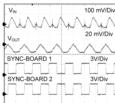
Figure 54. Output voltage ripple of two modules with synchronization clocks 180 degrees out of phase
