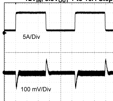
Transient response 12V IN , 3.3V OUT 1 to 10A Step
