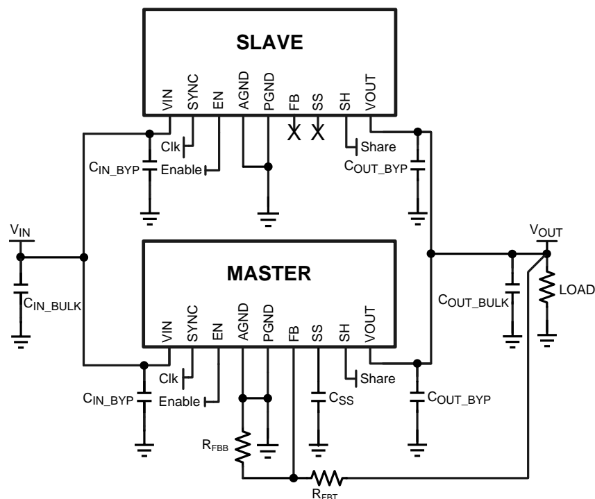
Figure 52. Current Sharing Example Schematic
