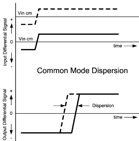
FIGURE 8. Common Mode Dispersion
