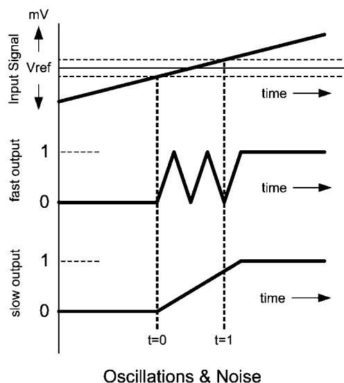
FIGURE 9. Oscillations &amp; Noise
