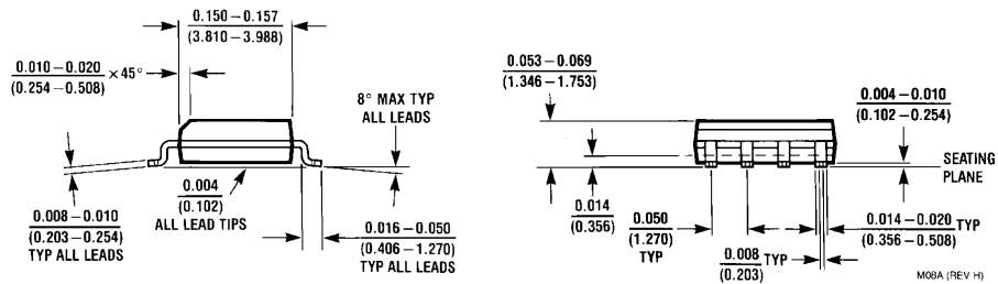
8-Pin Small Outline Package Order Number LMC6762AIM, LMC6762BIM, LMC6762AIMX or LMC6762BIMX NS Package Number M08A
