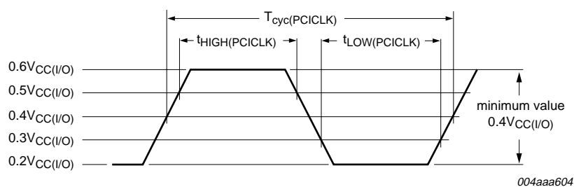
Fig 7. PCI clock
