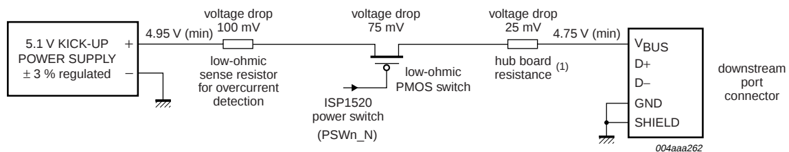
Fig 6. Typical voltage drop components in the self-powered mode using global overcurrent detection.
