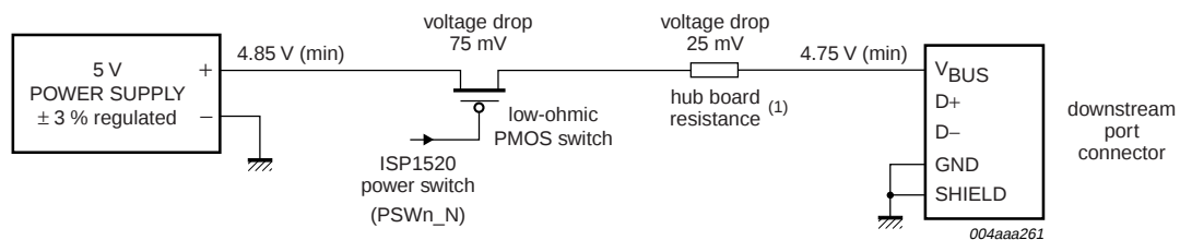
Fig 5. Typical voltage drop components in the self-powered mode using individual overcurrent detection.
