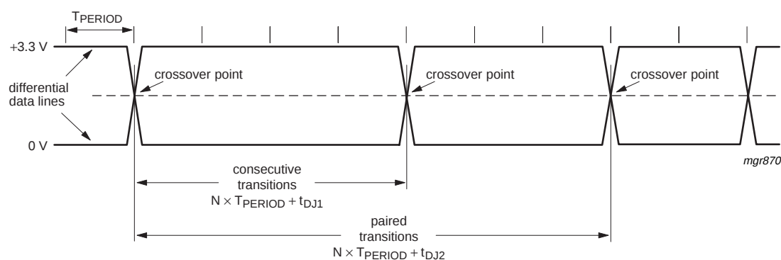
Fig 10. Source differential data jitter.
