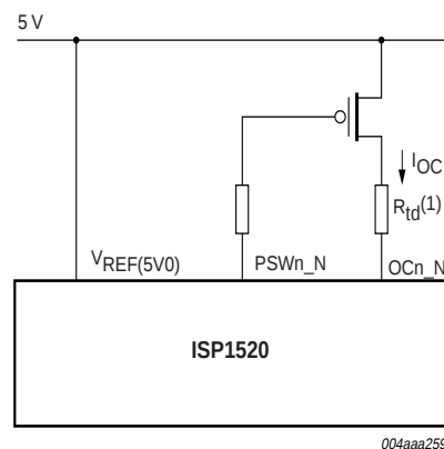
Fig 18. Adjusting analog overcurrent detection limit (optional).
