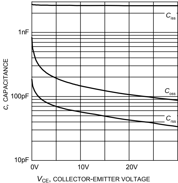
Figure 18. Typical capacitance as a function of collector-emitter voltage ( V_{GE}=0V , f=1\text{ MHz} )
