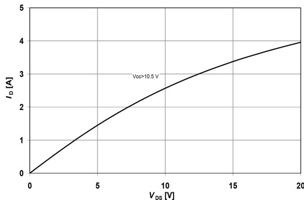
Figure 61 Typ. output characteristics; I_D=f(V_{DS}), T_J=150^\circ\text{C} , parameter: V_{CC}
