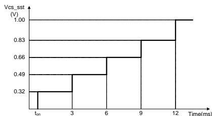
Figure 4 Maximum current sense voltage during softstart
