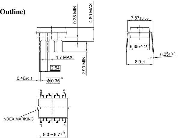
Figure 14 PG-DIP-8-6, PG-DIP-8-9 (Pb-free lead plating Plastic Dual-in-Line Outline)
