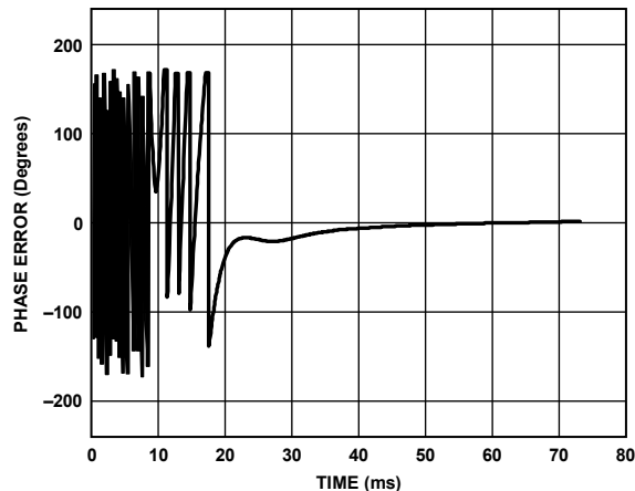
Figure 10. Phase Error During Lock Time for Divide by 5; 10 MHz Input; 50 MHz Output; Loop BW = 100 Hz; Refer to Loop Filter Configuration 2 in Table 5
