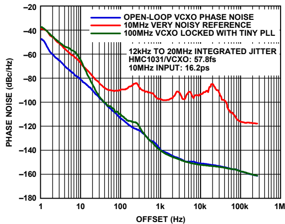
Figure 9. 10 MHz to 100 MHz with Very Noisy Reference Phase Noise; Loop Filter Value: C_8 = 4.7\text{ nF} , R_7 = 1.2\text{ k}\Omega , C_9 = 62\text{ }\mu\text{F} ; Loop Filter BW = 8 Hz; VCXO = 100 MHz Crystek CVHD-950
