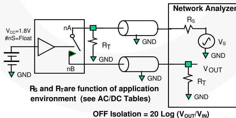
Figure 6. OFF Isolation
