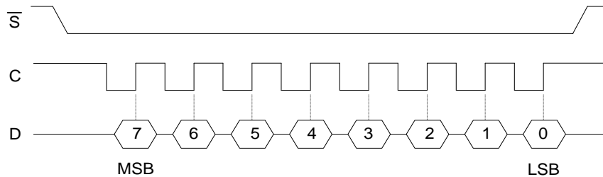
Figure 4. SPI Modes 0 & 3
