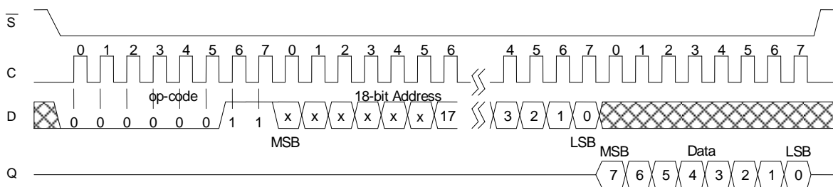
Figure 10. Memory Read
