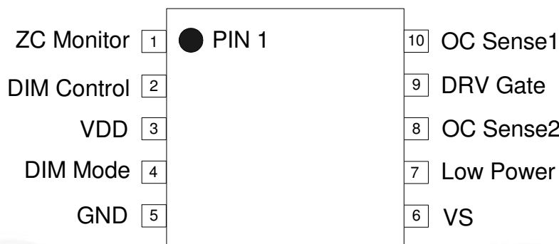
Figure 7. Pin Assignments
