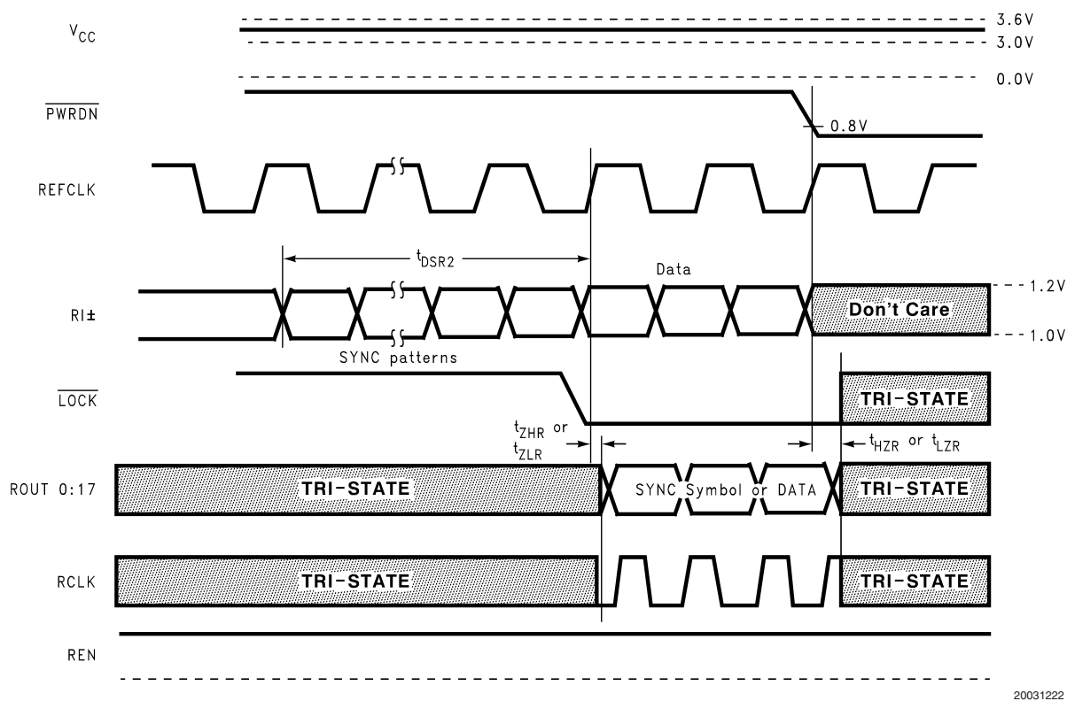
FIGURE 15. Deserializer PLL Lock Time from SYNC PAT
