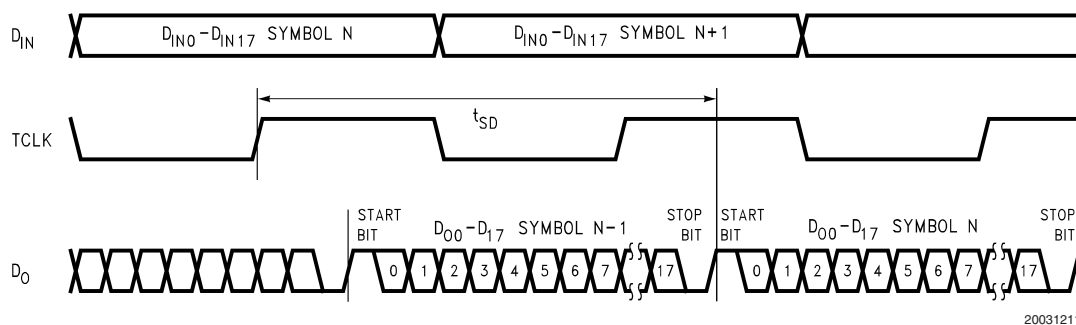
FIGURE 10. Serializer Delay
