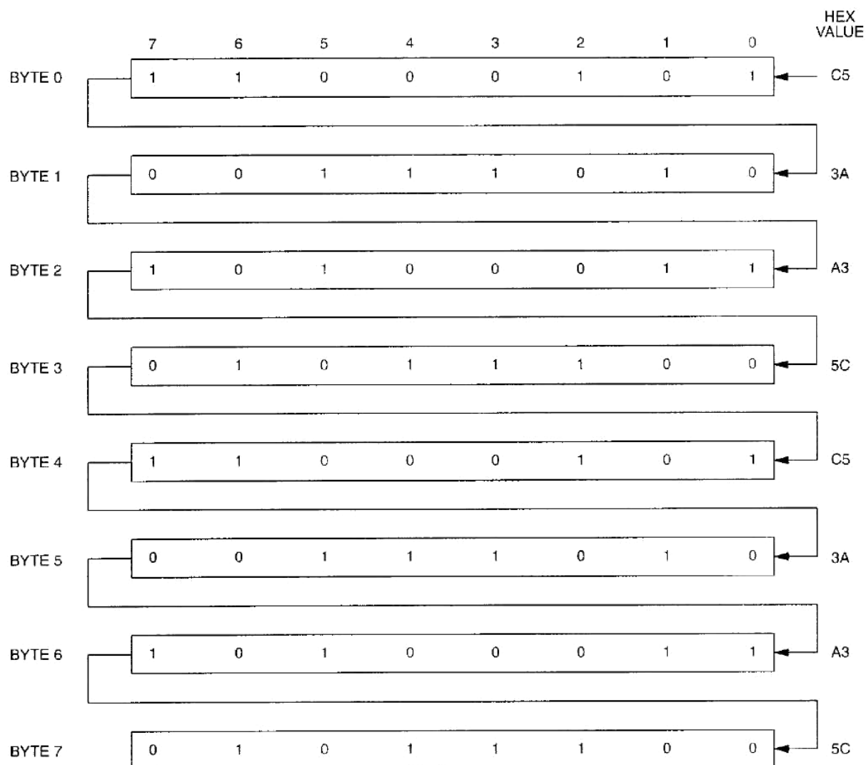
Figure 1. PHANTOM CLOCK REGISTER DEFINITION
