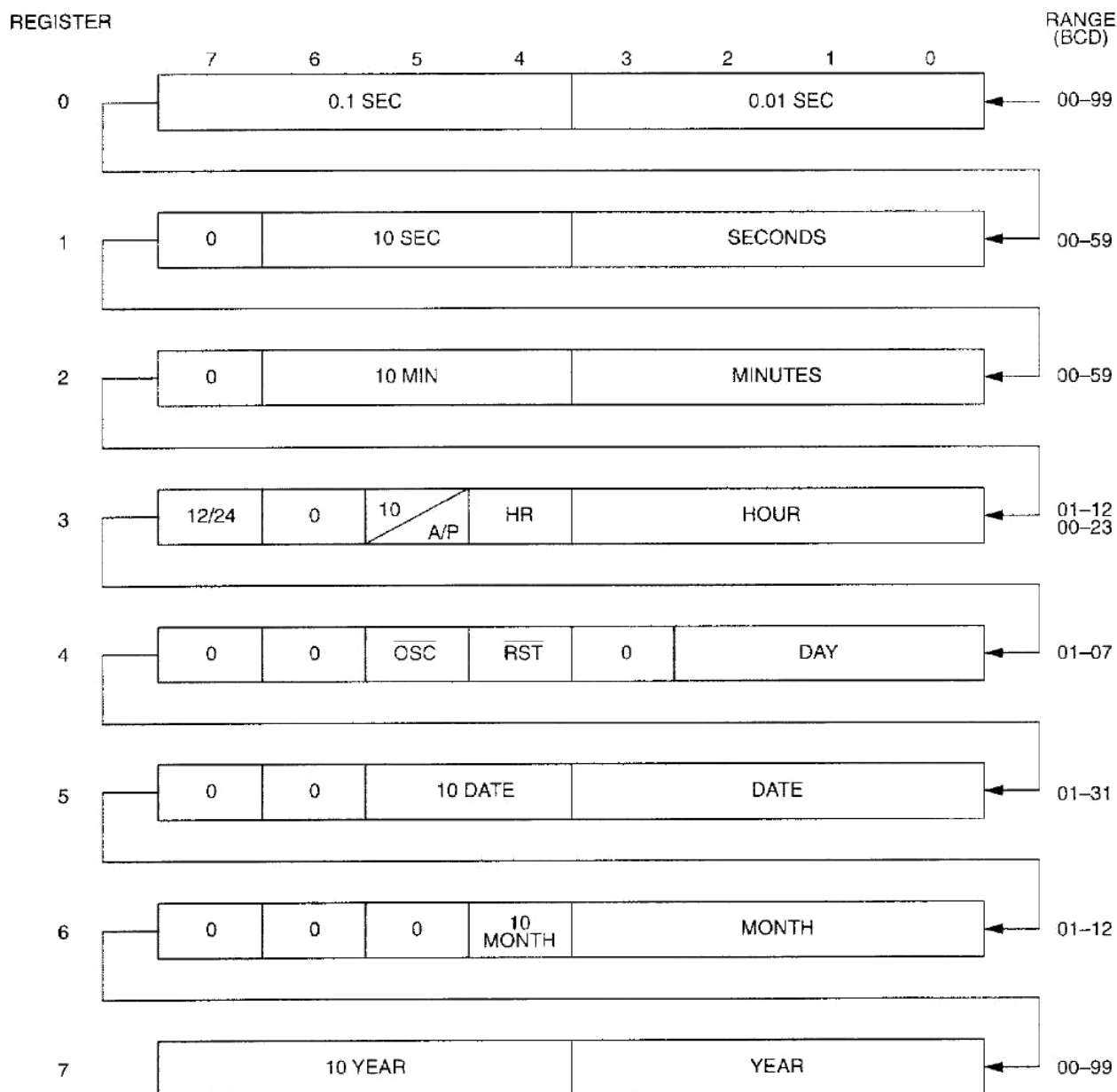
Figure 2. PHANTOM CLOCK REGISTER DEFINITION
