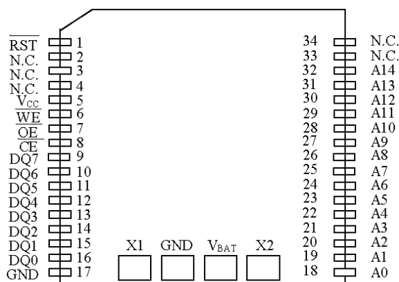
DS2144P 34-Pin PowerCap Module (Uses DS9034PCX PowerCap)
