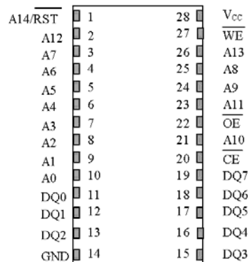
DS2144 28-PDIP Module(740mil)
