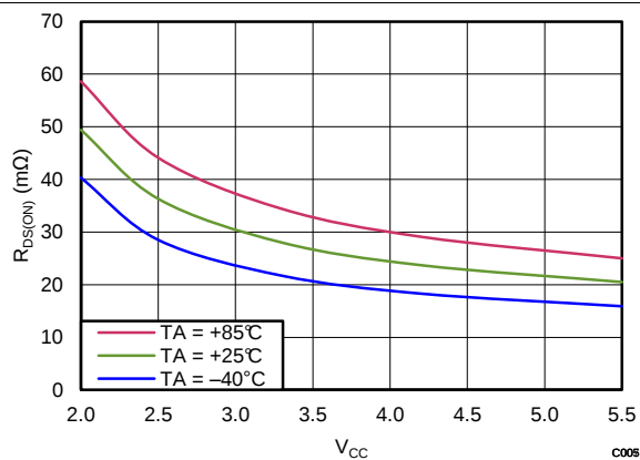
Figure 8. R_{DS(ON)} , LS – OUT2
