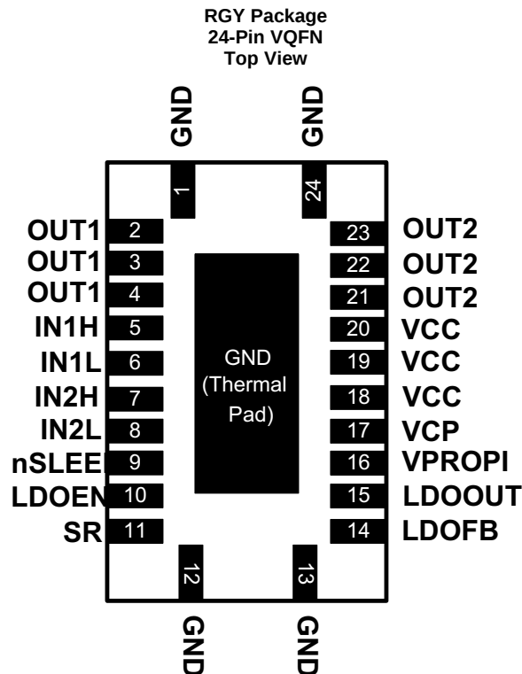
Pin Functions
