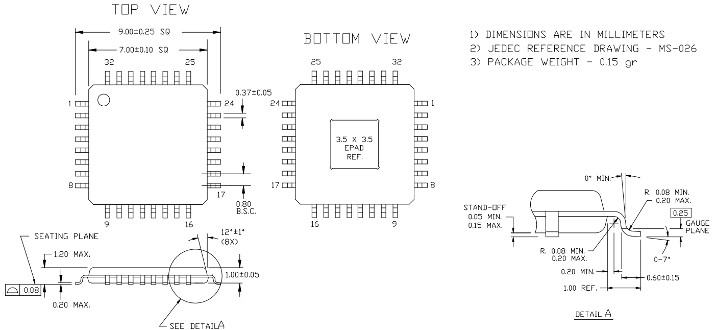
Figure 9. 32-Pin Thin Plastic Quad Flat Pack 7 × 7 × 1.0 mm
