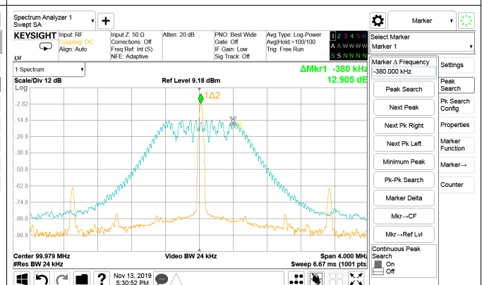
Figure 29. 100 MHz With +/- 0.5% Center Spread With and Without Trace
