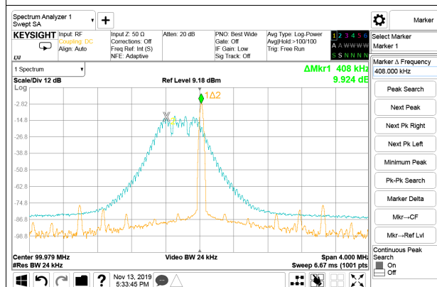
Figure 28. 100 MHz With -0.5% Down Spread With and Without Trace
