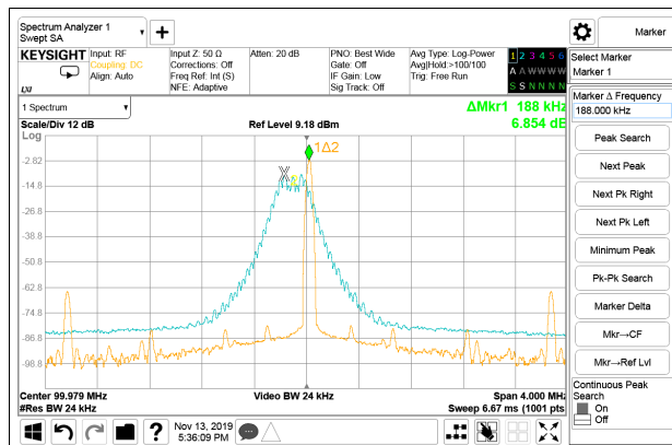
Figure 26. 100 MHz With -0.25% Down Spread With and Without Trace
