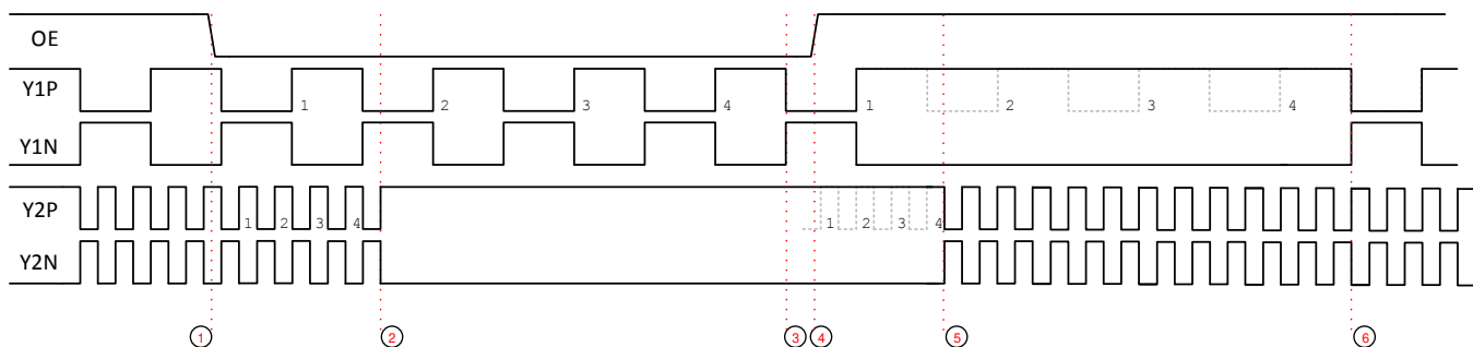
Figure 32. Individual Output Enable and Disable
