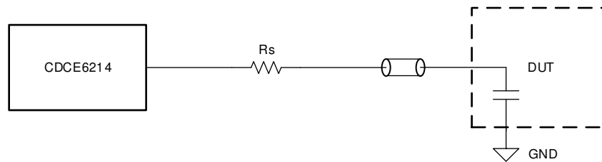
Figure 19. LVCMOS Output
