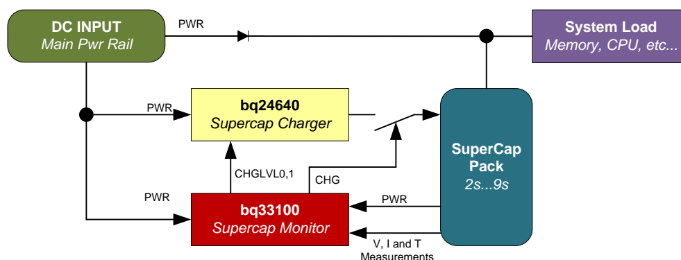
bq33100 System Diagram
