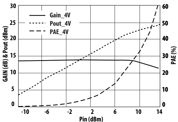
Figure 18. Small Signal Gain/Pout/PAE vs. P_{in} at V_{ds}=3V and Freq= 2\text{ GHz}
