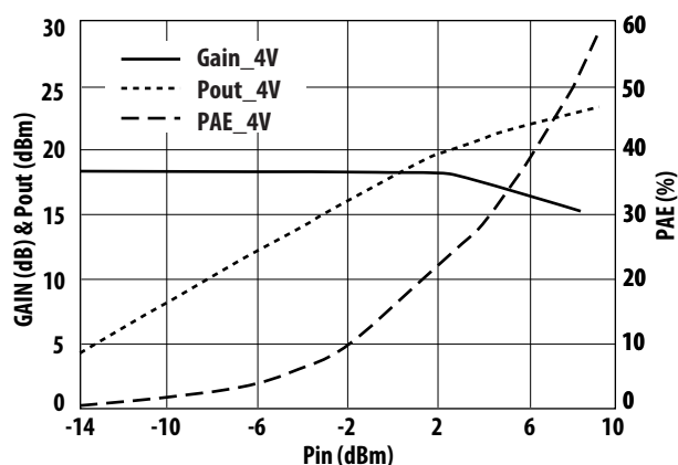
Figure 16. Small Signal Gain/Pout/PAE vs. P_{in} at V_{ds}=4V and Freq=900\text{ MHz}
