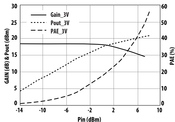
Figure 15. Small Signal Gain/Pout/PAE vs. P_{in} at V_{ds}=3V and Freq=900\text{ MHz}
