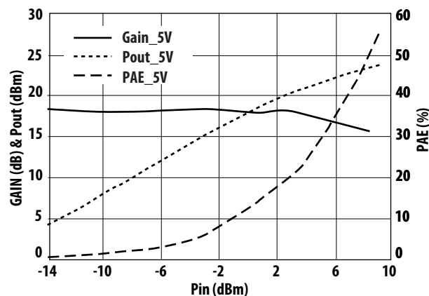
Figure 17. Small Signal Gain/Pout/PAE vs. P_{in} at V_{ds}=5V and Freq=900\text{ MHz}
