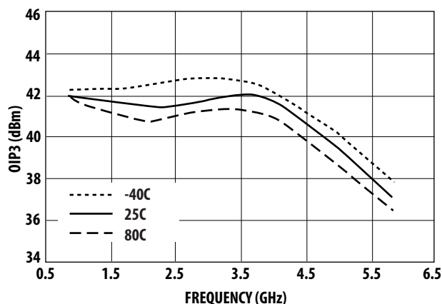
Figure 27. OIP3 vs. Temperature and Frequency at optimum OIP3
