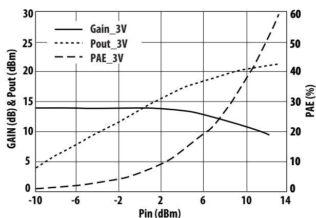
Figure 20. Small Signal Gain/Pout/PAE vs. Pin at V_{ds}=5V and Freq = 2 GHz
