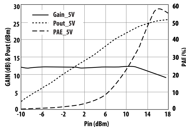
Figure 23. Small Signal Gain/Pout/PAE vs. Pin at V_{ds}=5V and Freq=3.9 GHz
