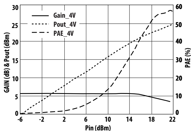
Figure 25. Small Signal Gain/Pout/PAE vs. Pin at V_{ds}=4V and Freq=5.8\text{ GHz}
