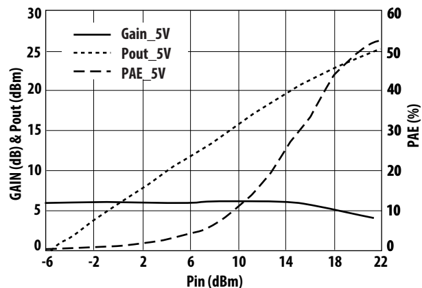
Figure 26. Small Signal Gain/Pout/PAE vs. Pin at V_{ds}=5V and Freq=5.8\text{ GHz}
