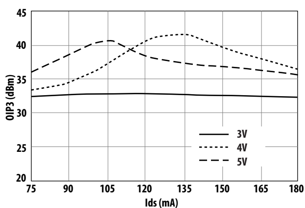
Figure 8. OIP3 vs. I_{ds} and V_{ds} at 2 GHz
