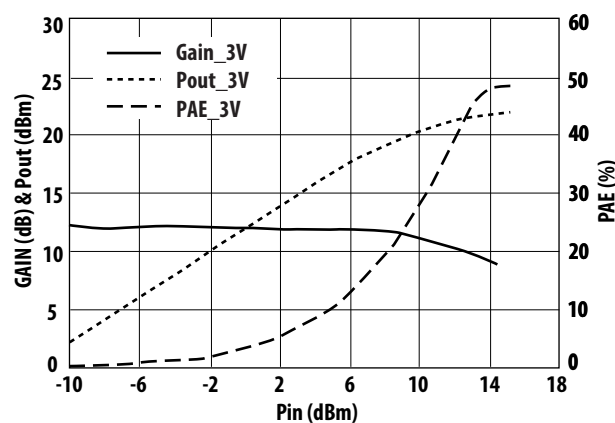
Figure 21. Small Signal Gain/Pout/PAE vs. Pin at V_{ds}=3V and Freq=3.9 GHz
