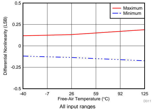
Figure 23. DNL vs Temperature
