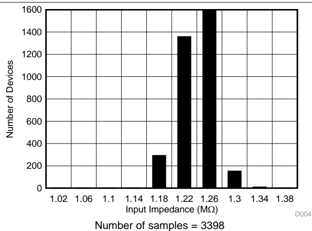
Figure 12. Typical Distribution of Input Impedance
