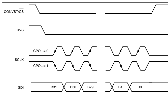
Figure 75. Standard SPI Timing Protocol (CPHA = 0, 32 SCLK Cycles)
