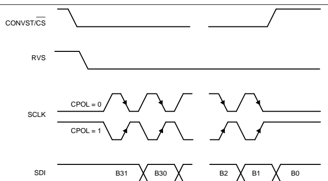
Figure 76. Standard SPI Timing Protocol (CPHA = 1, 32 SCLK Cycles)
