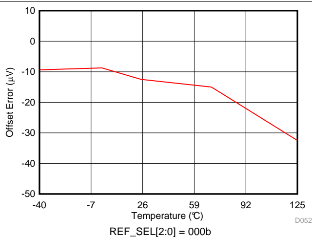
Figure 14. Offset Error vs Temperature
