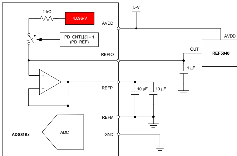
Figure 36. Device Connections for Using an External Reference
