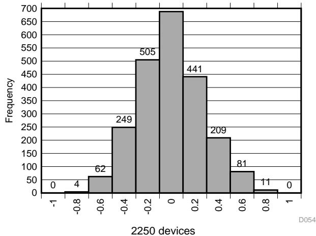
Figure 12. Typical Offset Distribution (LSB)
