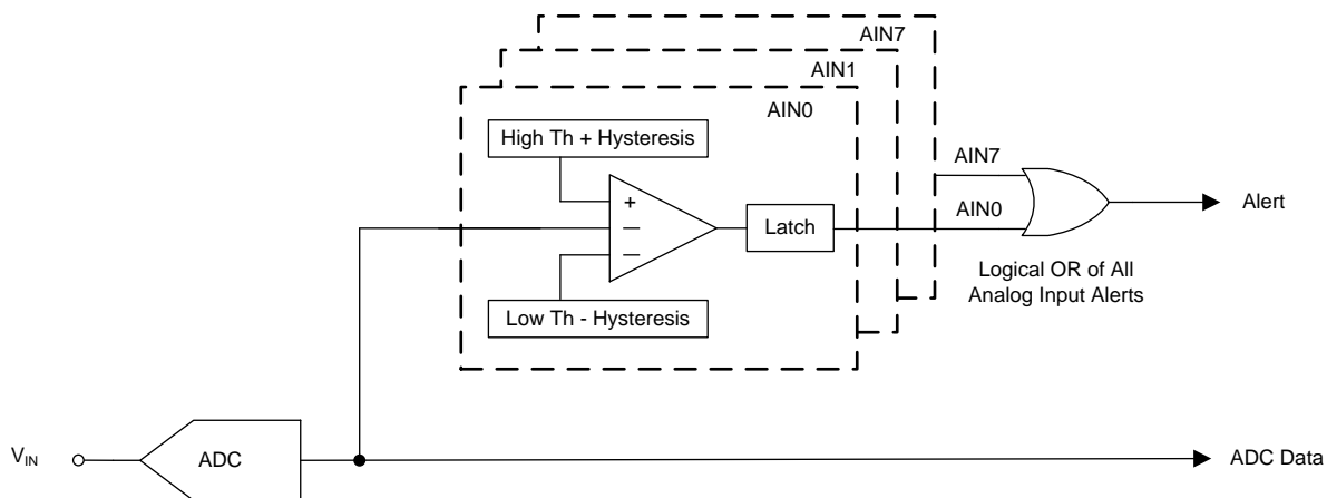
Figure 49. Digital Window Comparator
