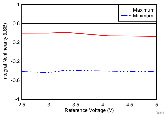
Figure 11. INL vs Reference Voltage
