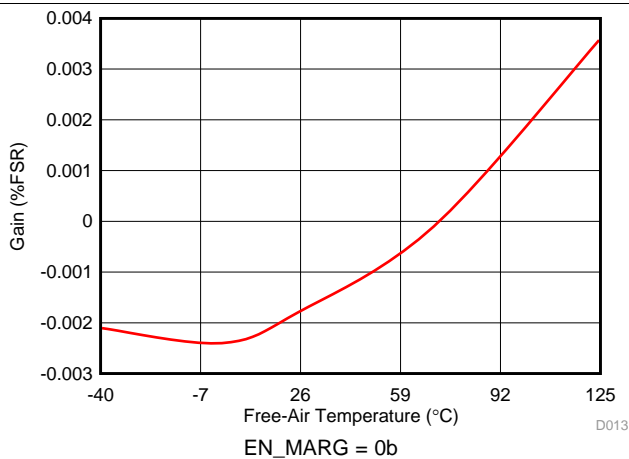
Figure 16. Gain Error (ADC + REFBUF) vs Temperature
