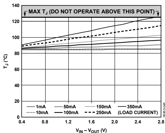
Figure 46. TSOT, T A = 85°C
