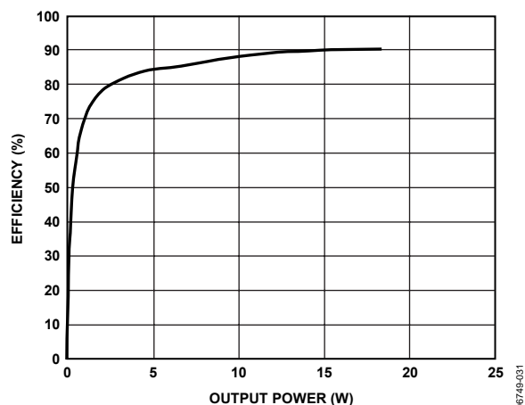
Figure 31. Efficiency vs. Output Power, 15 V, 8 \Omega
