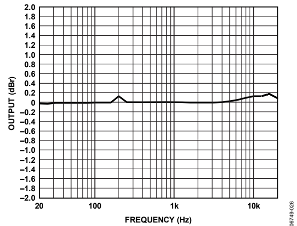
Figure 26. Frequency Response @ 1 W, 6 \Omega , PVDD = 15 V, PGA = 0 dB
