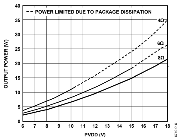
Figure 16. Output Power vs. PVDD @ 10% THD + N
