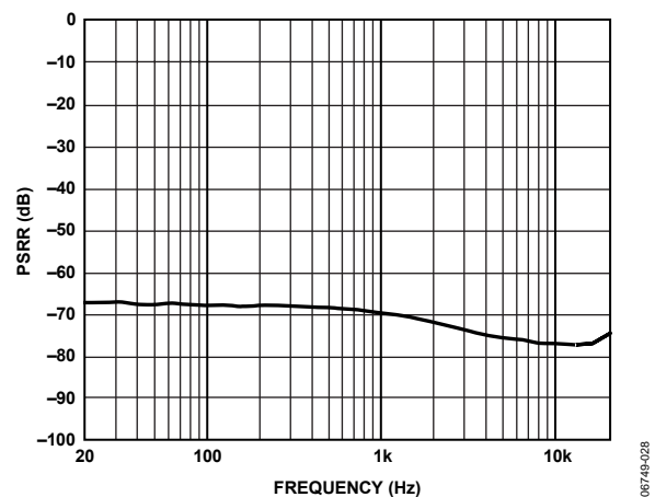
Figure 28. PSRR vs. Frequency, No Input Signal, Ripple = 1.5 V p-p, PVDD = 15 V, 6 \Omega
