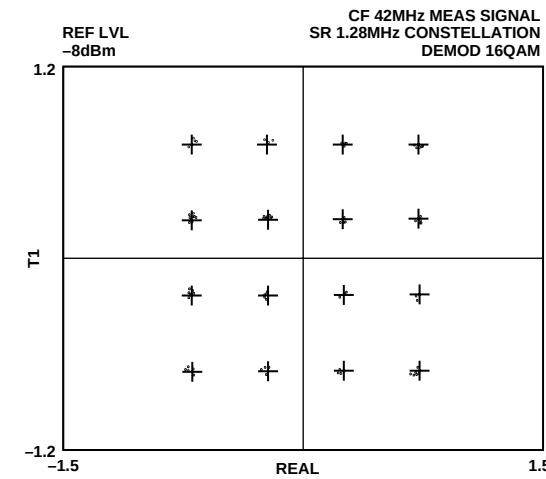
Figure 19. 16-QAM Modulation
