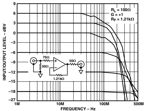
TPC 17. Large Signal Frequency Response, G = +1
